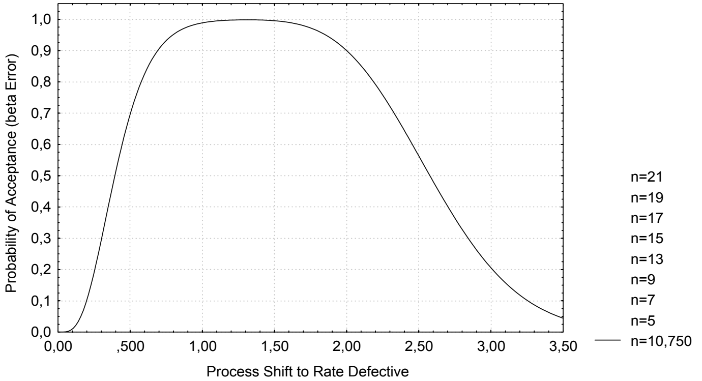
Operating Characteristic Curve for U-CHART; DISCONFO Control Limits: UCL=3,0000*S LCL=-3,0000*S
