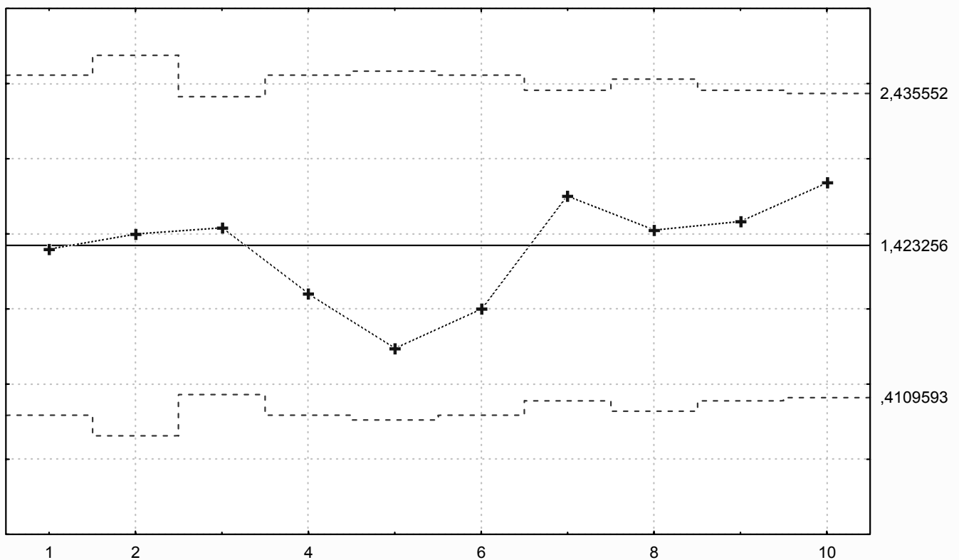
U Chart Mean: 1,42326 (1,42326) Sigma: ,363862 (,363862) n: 10,75
